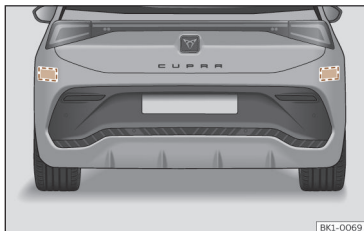
Fig. 98 Rear view of the vehicle: radar sensor zones.
