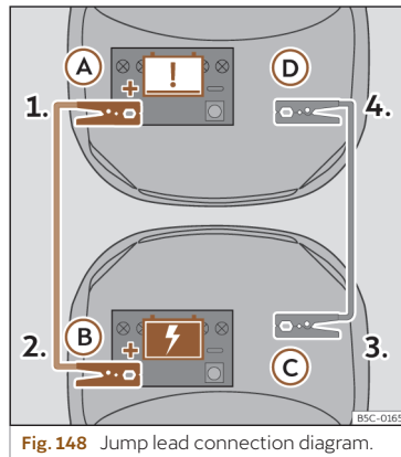
Fig. 148 Jump lead connection diagram.
